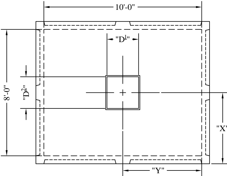
PLAN VIEW
