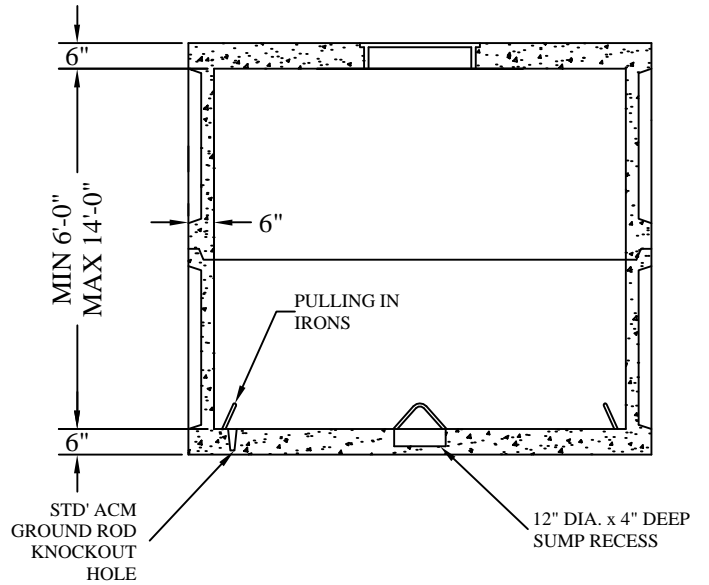
SECTION VIEW
